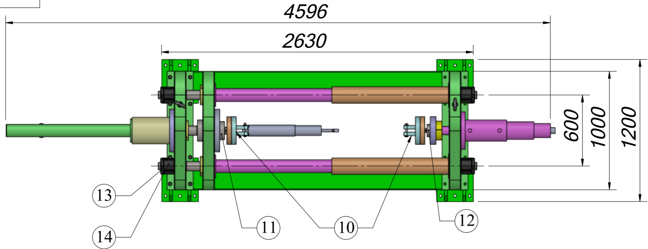
TOP VIEW
