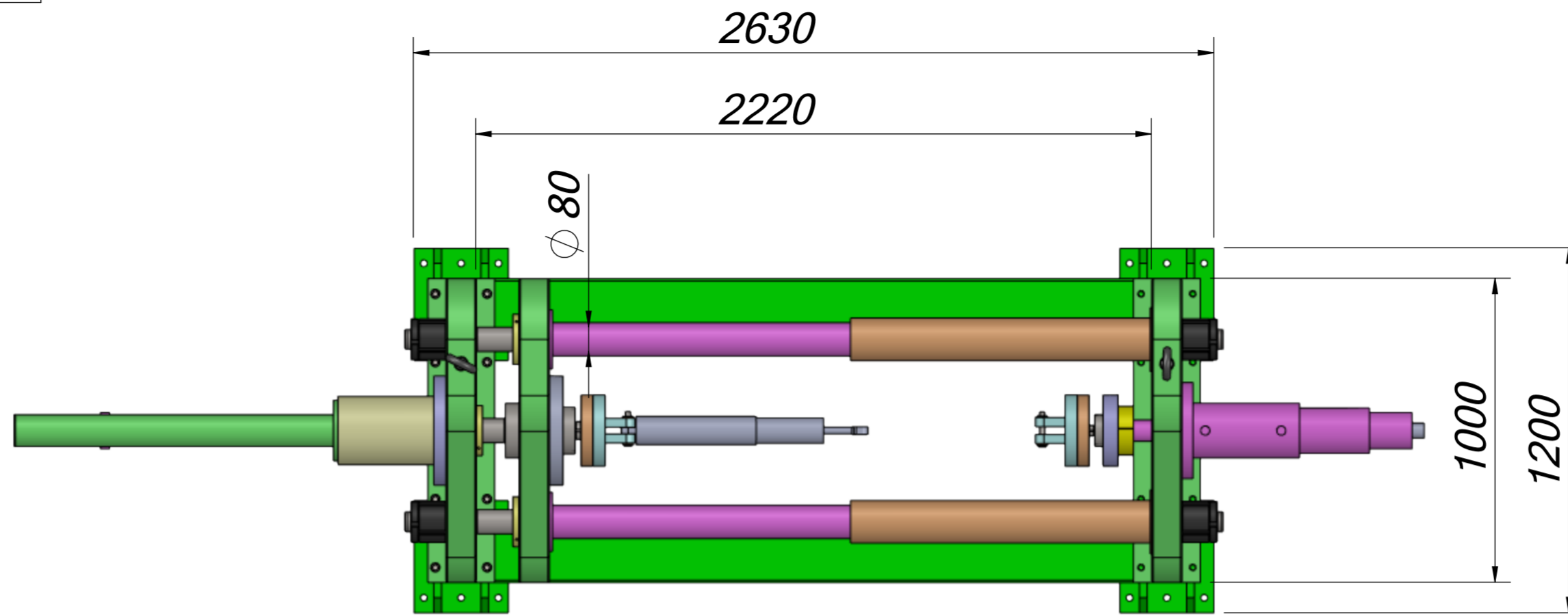
TOP VIEW
