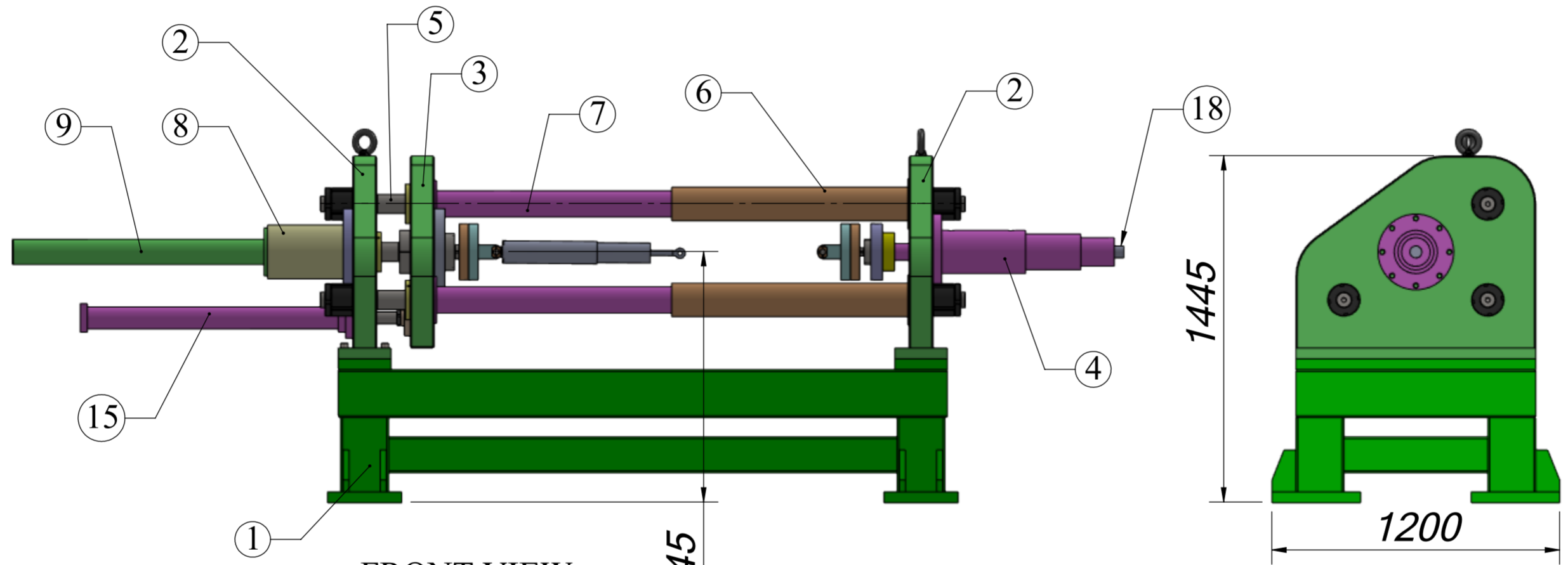
FRONT VIEW
