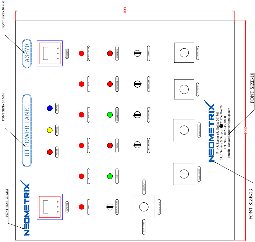
PANEL PRINTING DRAWING
