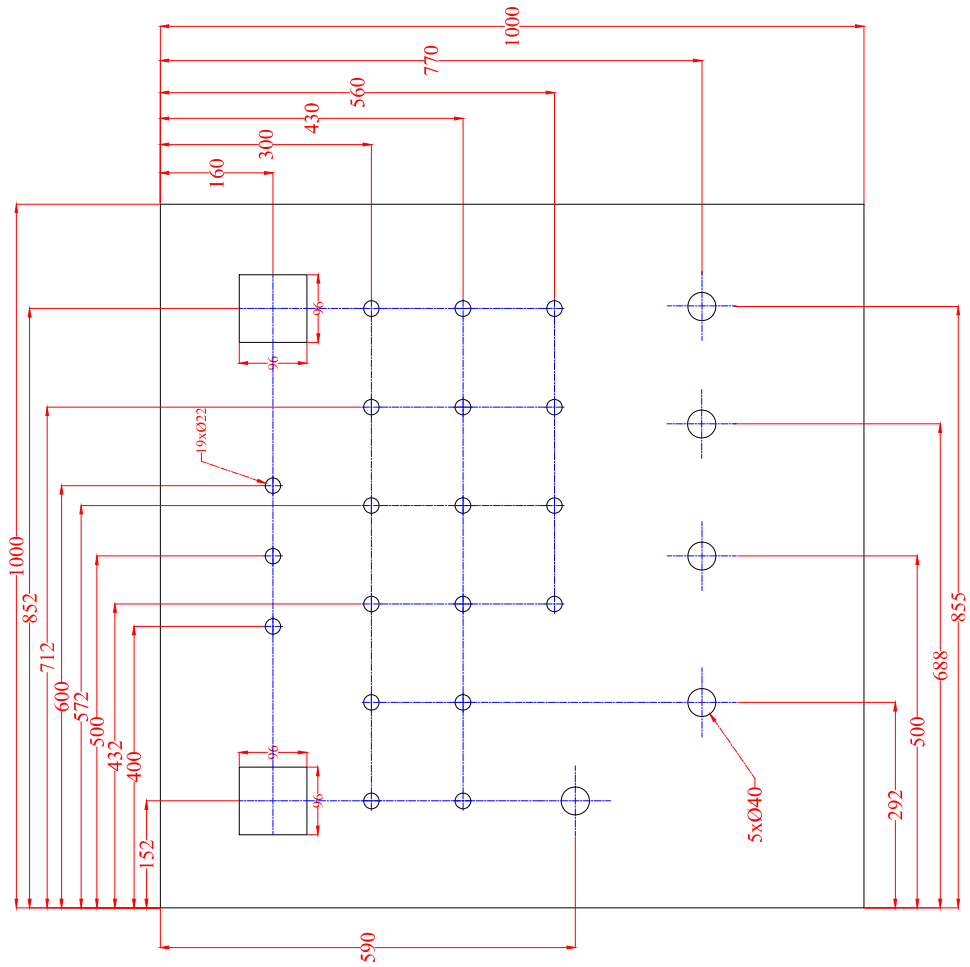
CUTOUT DRAWING
