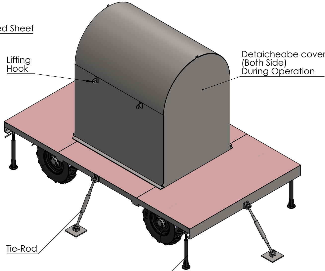
ISOMETRIC VIEW
