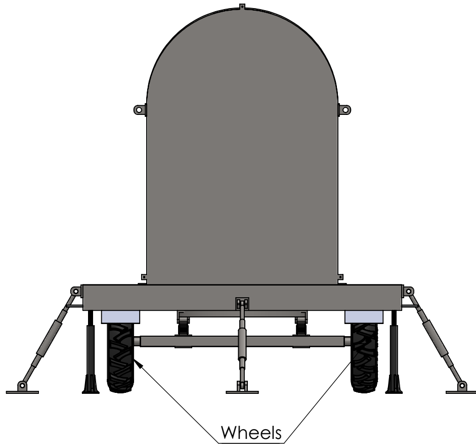
RIGHT VIEW
