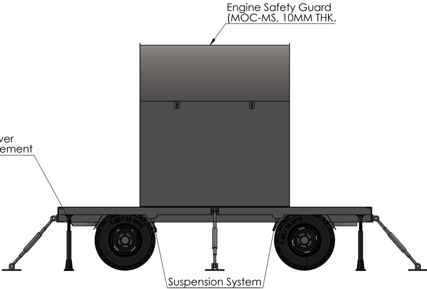
FRONT VIEW
