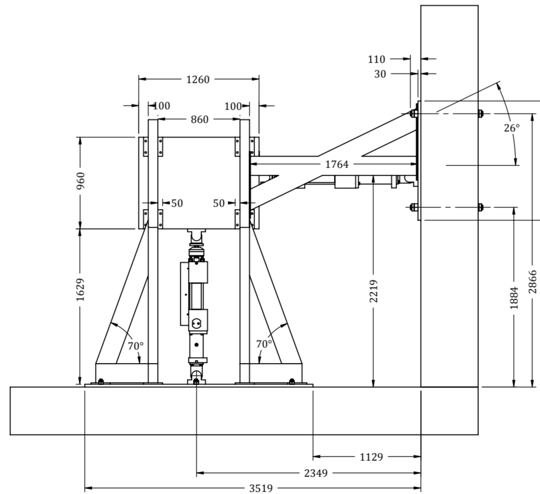
SIDE VIEW (SCALE 1 : 40)
