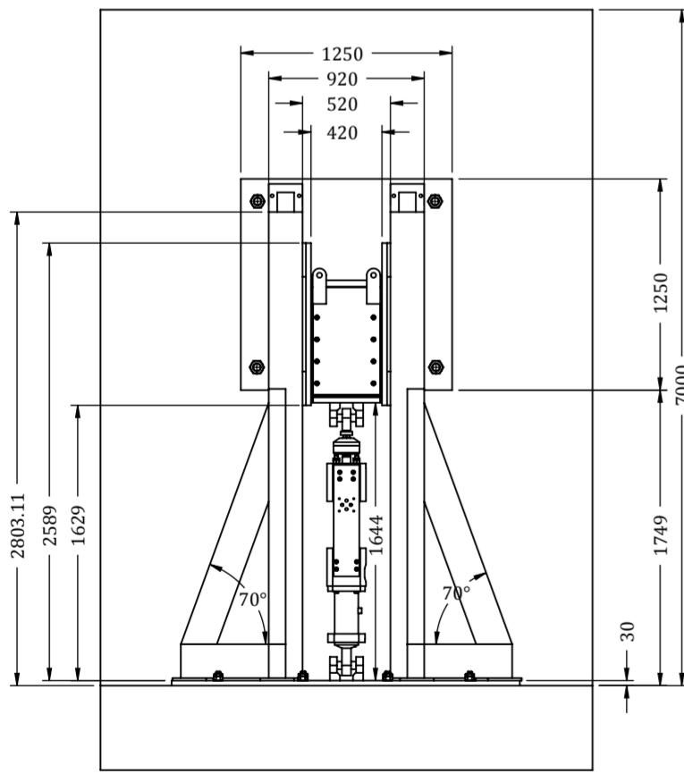
FRONT VIEW (SCALE 1 : 40)
