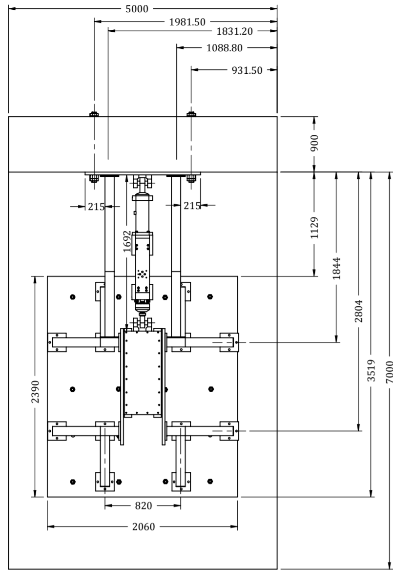
TOP VIEW (SCALE 1 : 40)
