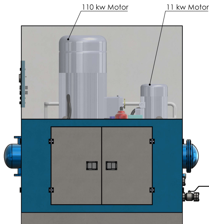
FRONR VIEW
