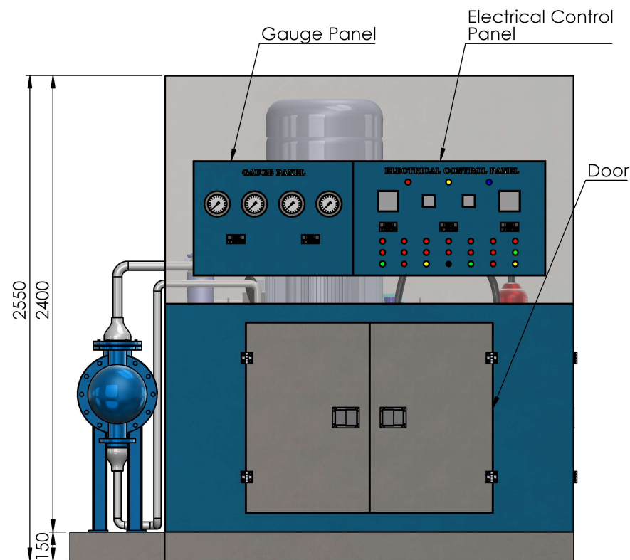
LEFT VIEW
