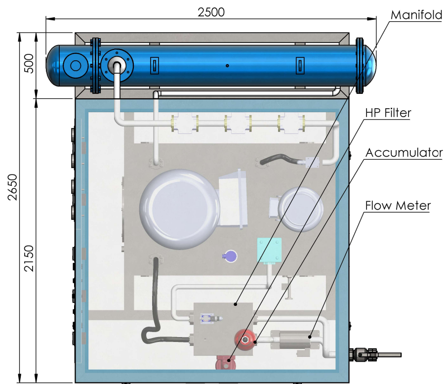
TOP VIEW
