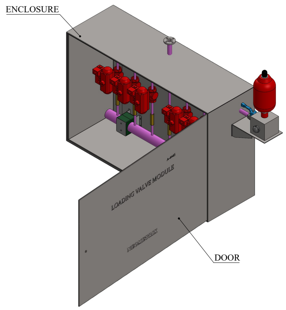
ISOMETRIC VIEW
