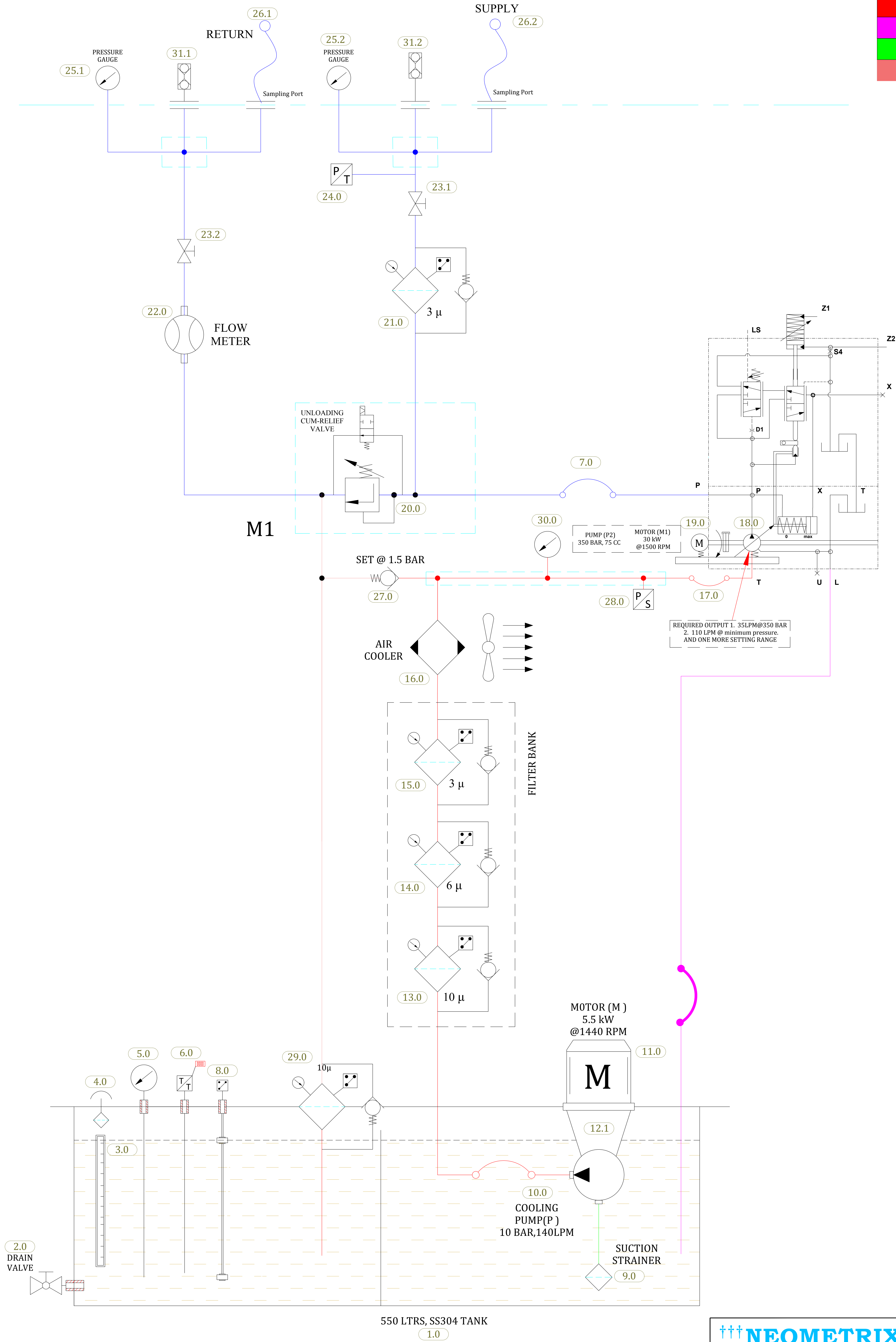
Hydraulic Flushing Rig
