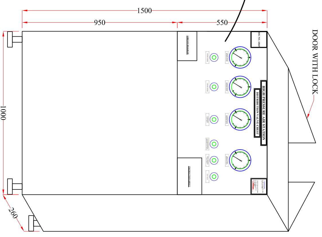
GA DRAWING (NOT TO DIMENSION)
