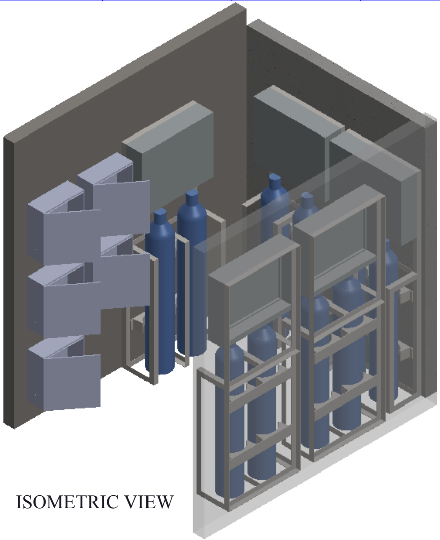
GAS BANK AREA
