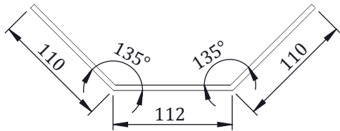
BRACKET BACK SUPPORT DETAIL MATERIAL:SS QTY: 4 Nos
