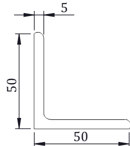
STRUCTURAL MEMBER DETAIL
