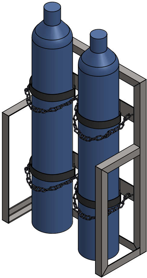
ISOMETRIC VIEW
