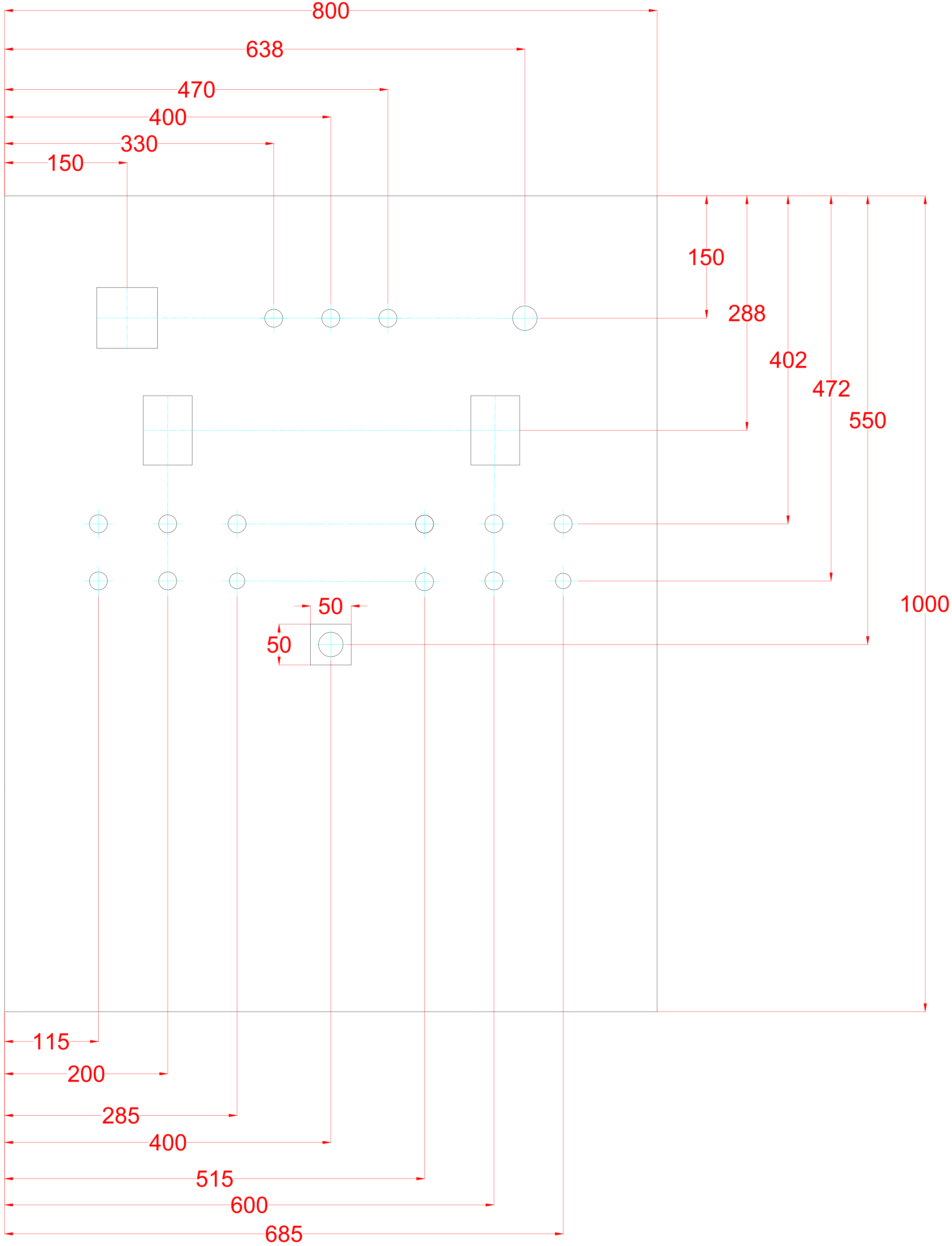
CUTOUT DRAWING
