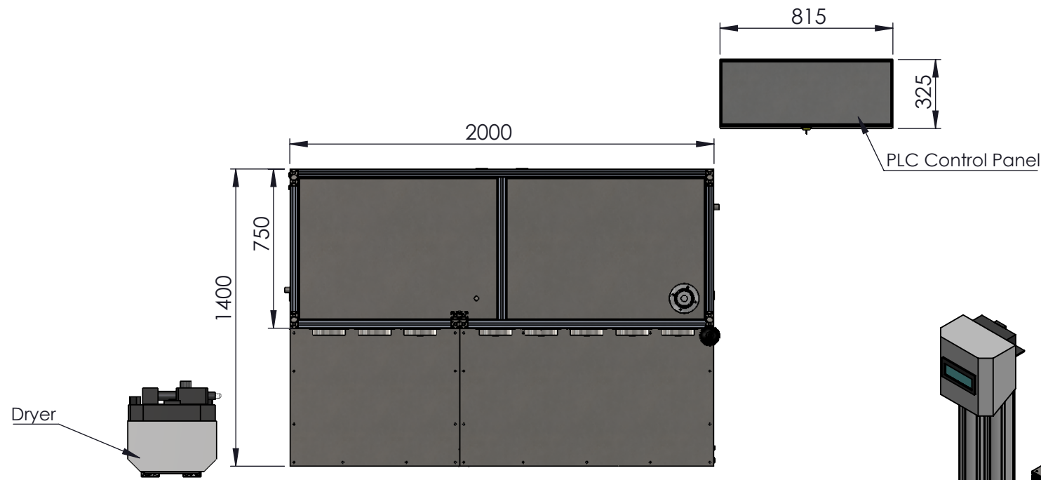
TOP VIEW
