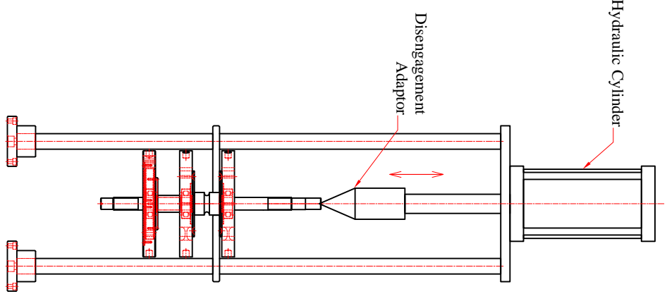
Step-2 Disc-1 Disengagement
