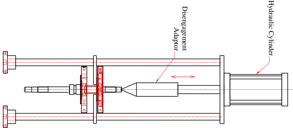
Step-3 Disc-3 Disengagement
