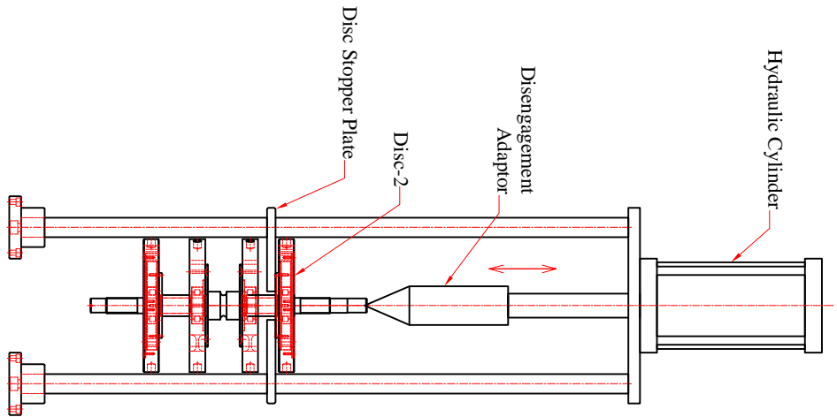
Step-1 Disc-2 Disengagement
