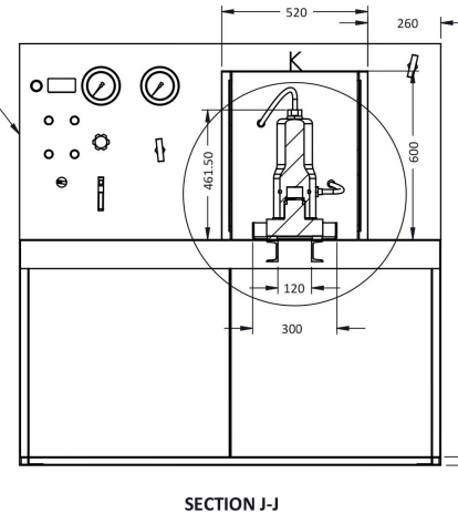
SECTION J-J
