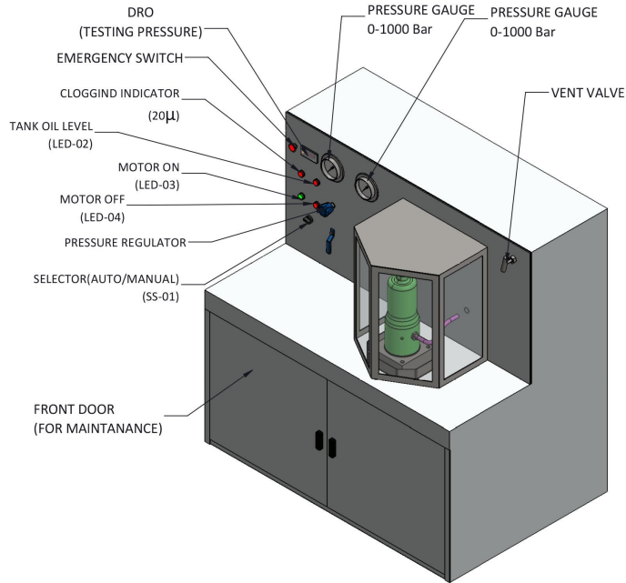
ISOMETRIC VIEW
