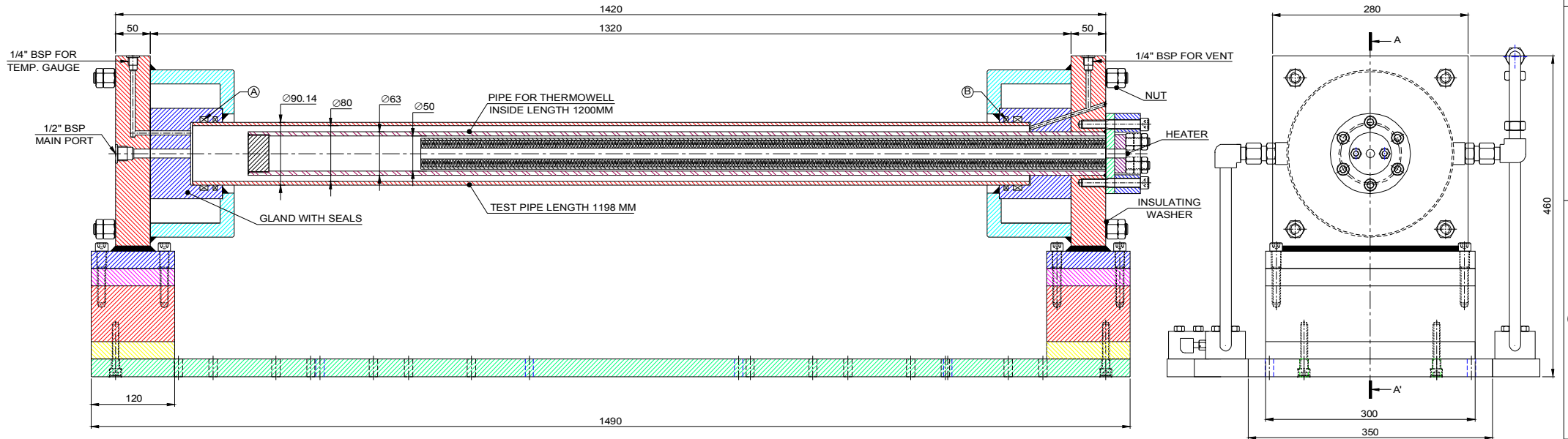
SECTION VIEW OF A-A'
