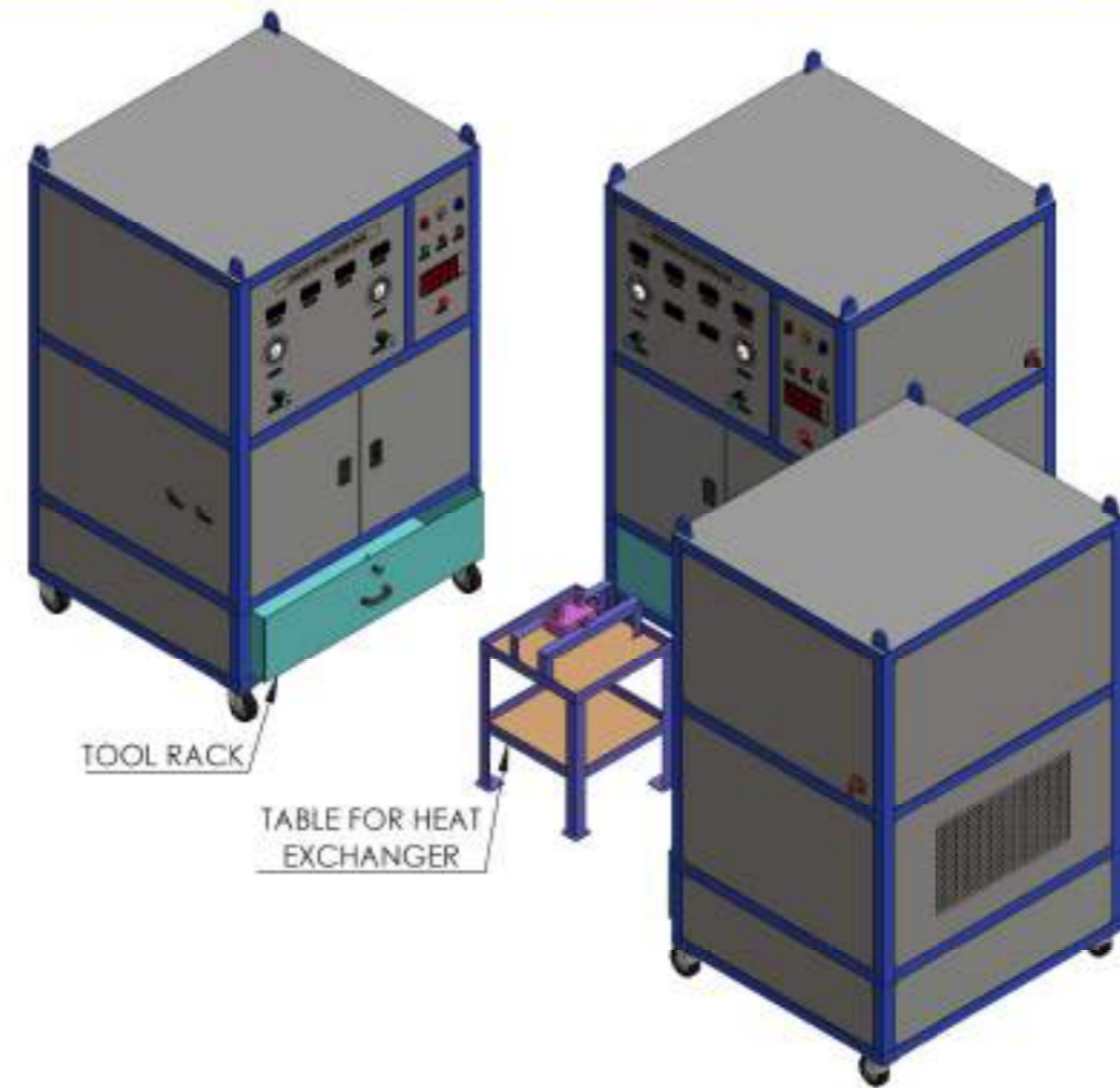
ISOMETRIC VIEW
