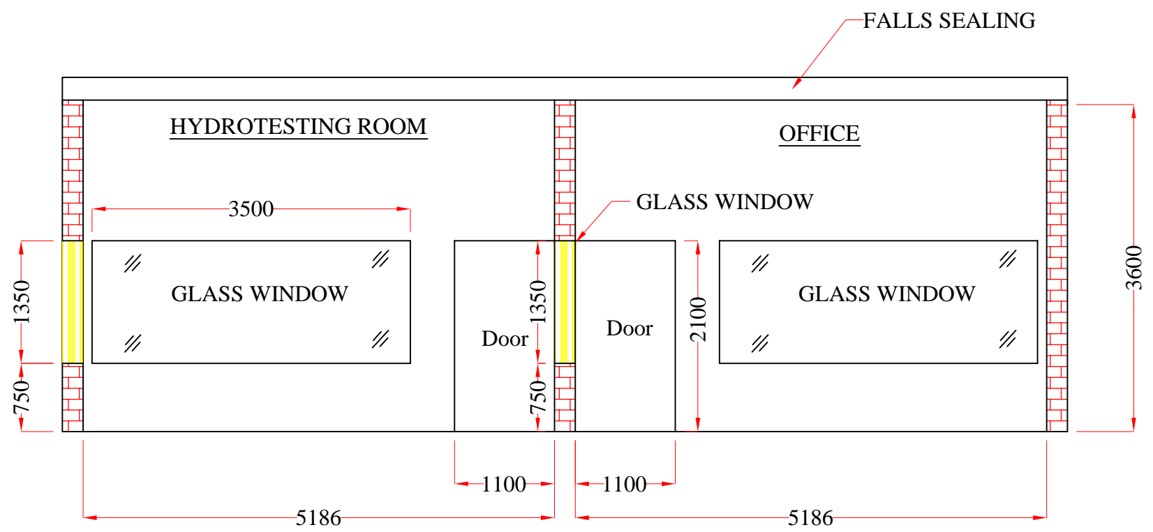
DETAIL OF ROOM HEIGHT (HYDRO TESTING & OFFICE)
