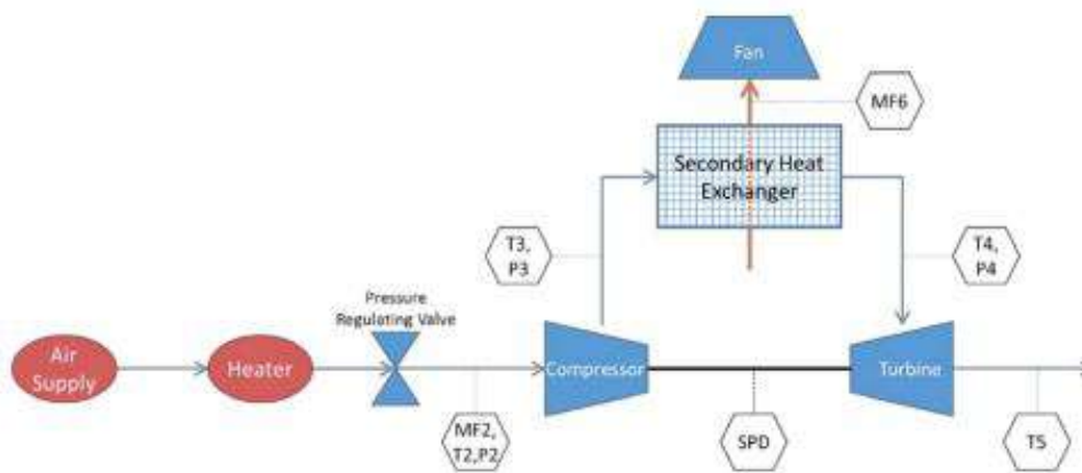
Fig. 6 ACM test bench with locations of observed variables identified [29]
