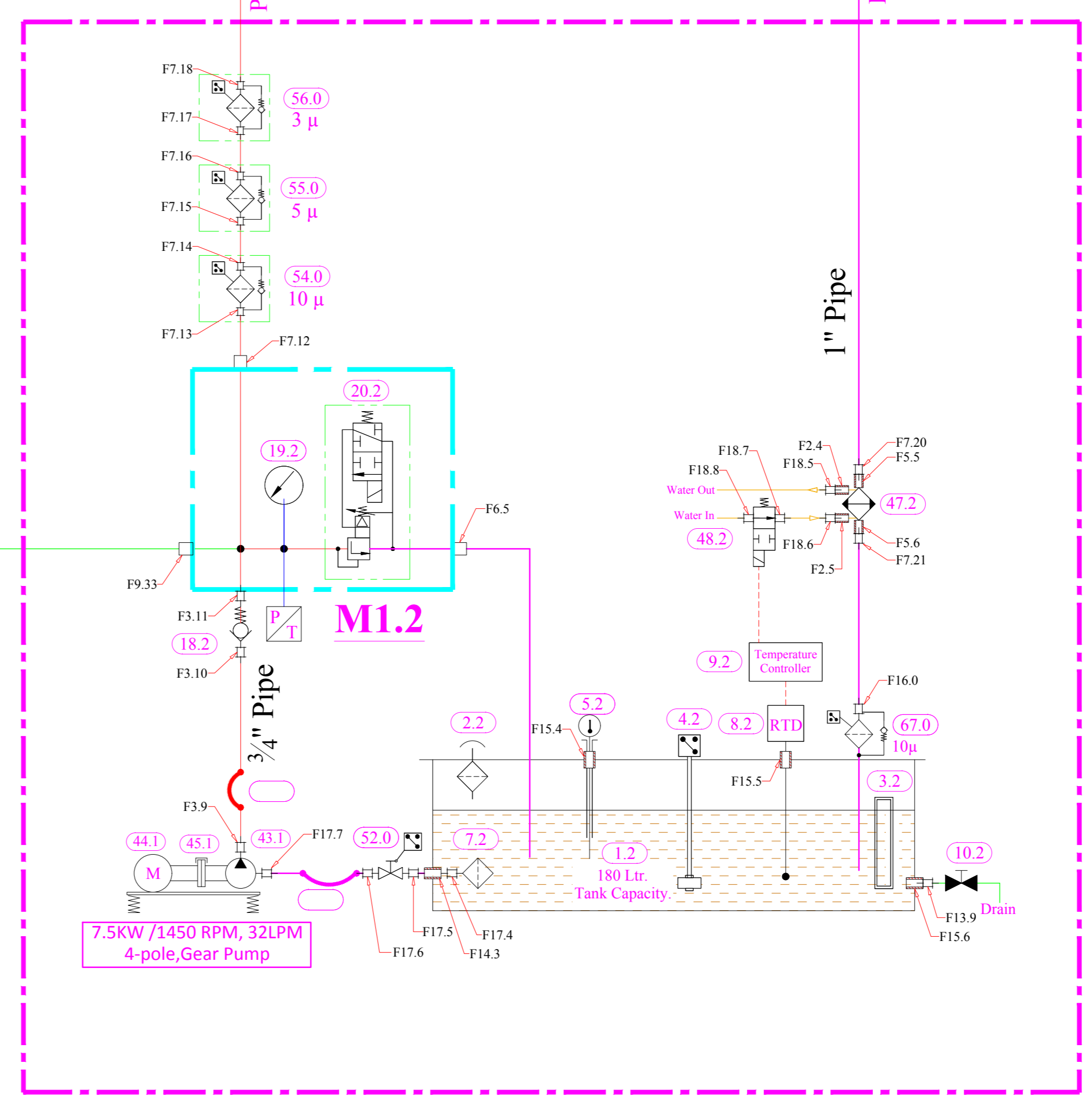
FLUSHING SYSTEM
