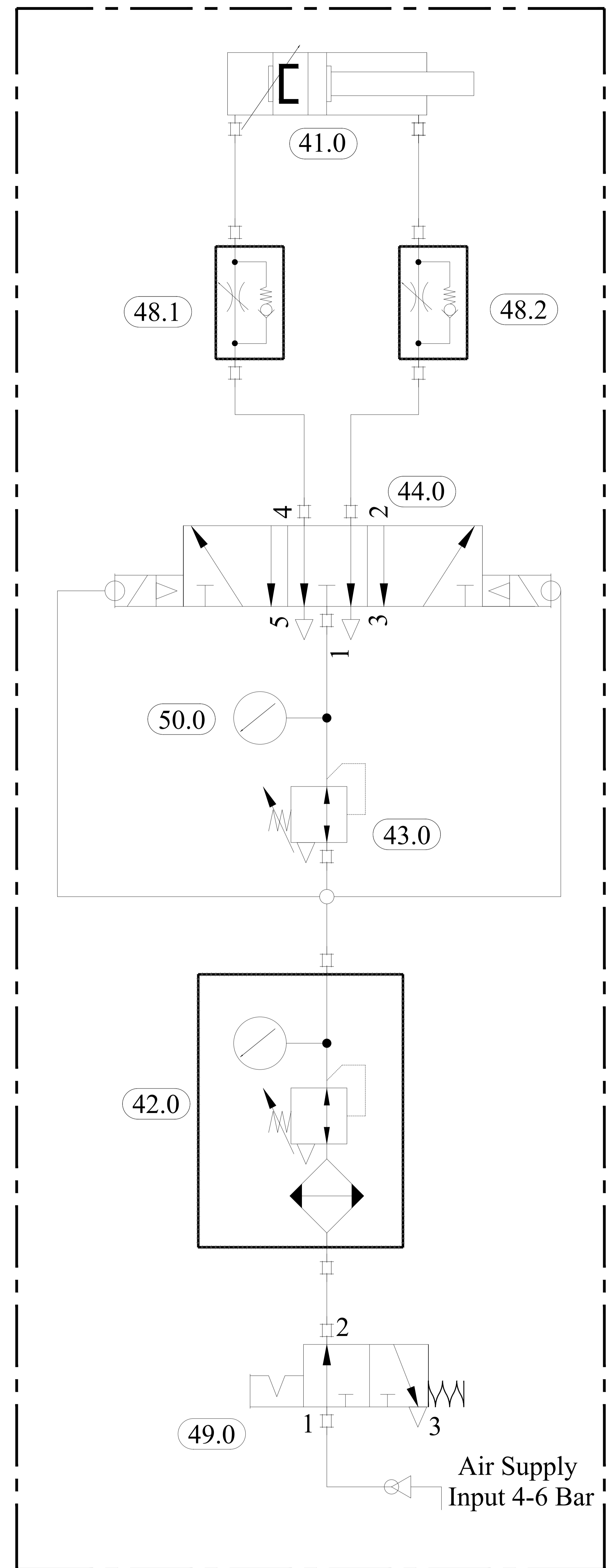
Pneumatic Circuit for Actuator
