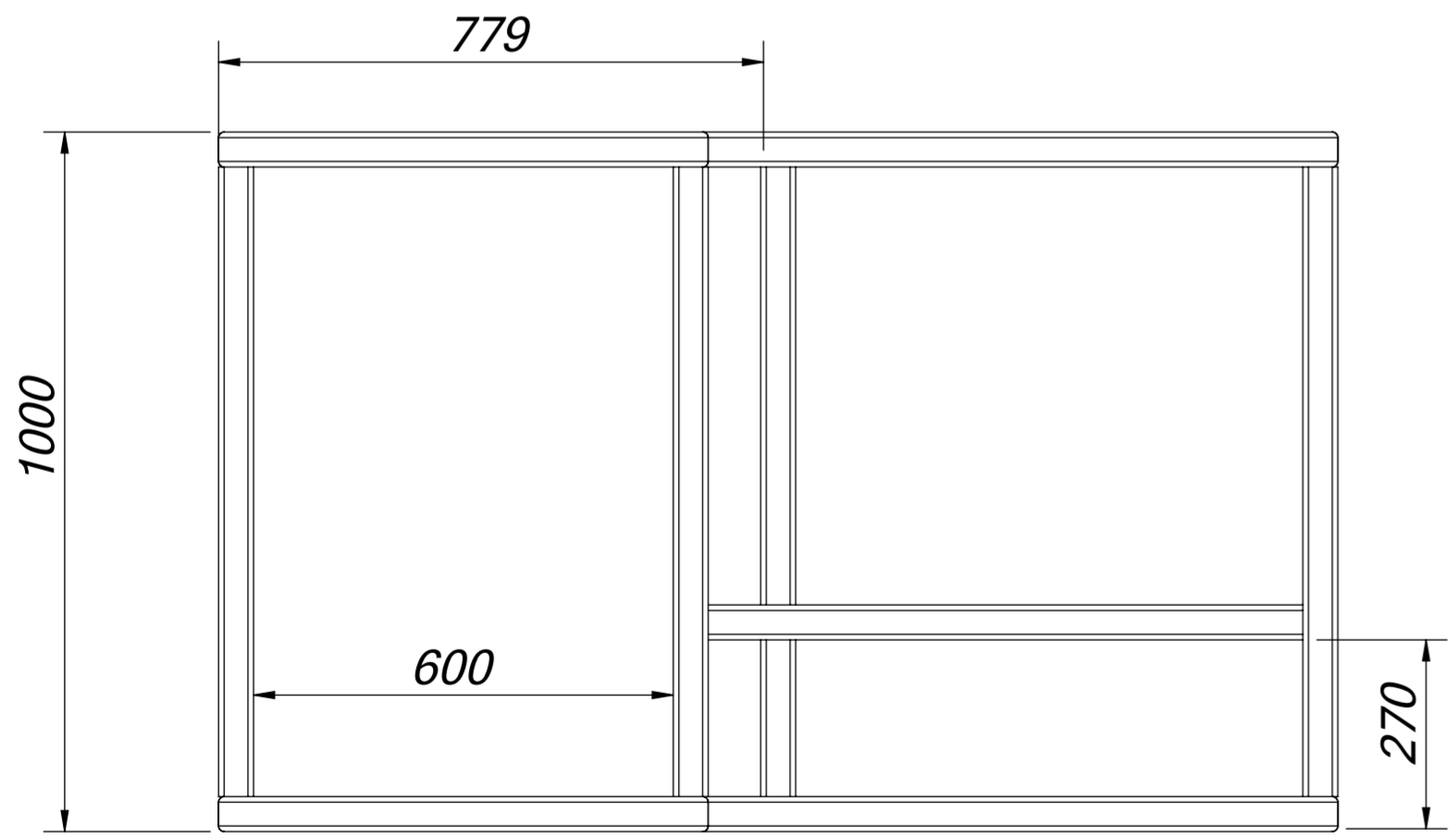
FRONT VIEW
